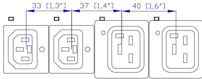
VIEW B
