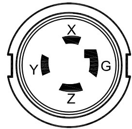
NEMA L15-30P PSE VIEW A
