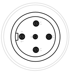
CLIPSAL 56P532
