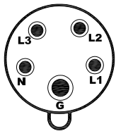
IEC60309 60/63A 3PY
