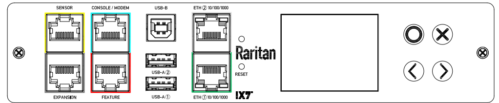
VIEW C
