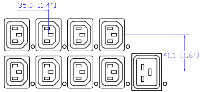
VIEW B
