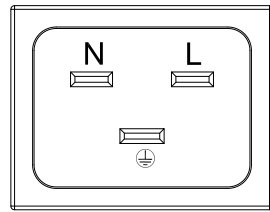
IEC 320 C20
